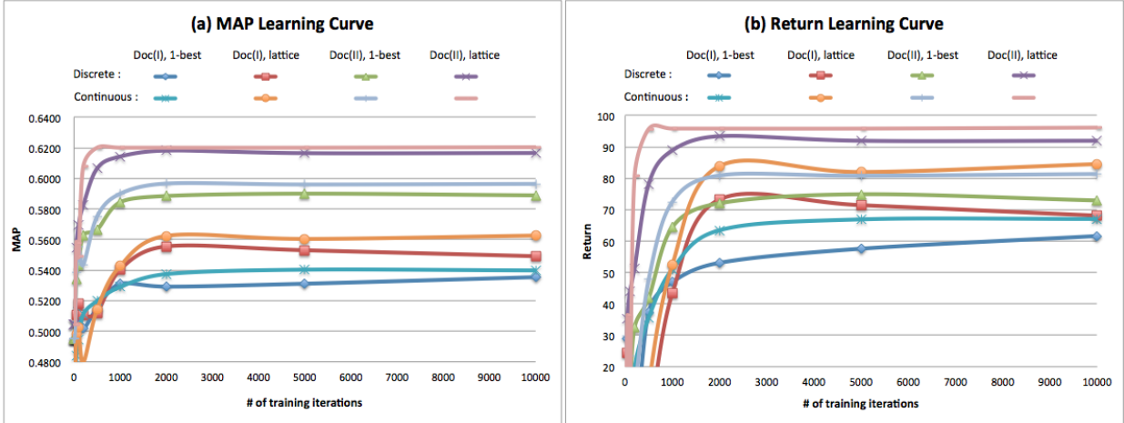
Fig. 2: (a) Mean Average Precision (MAP) and (b) Return for the proposed approach with estimated states for discrete/continuous state space MDP for the two recognition conditions Doc (I) and (II) , 1-best and lattices, under different number of training iterations.
