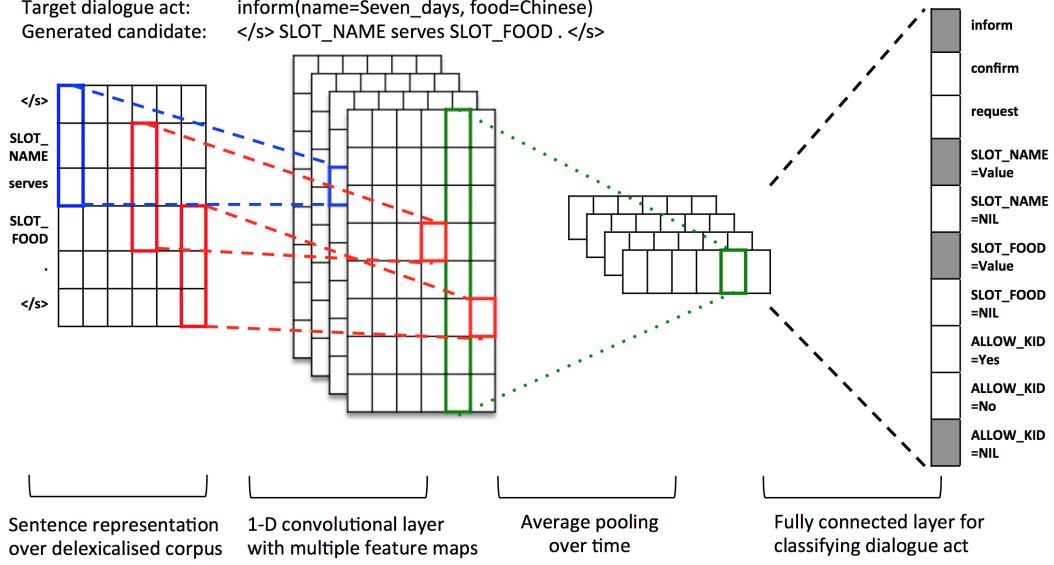
Figure 2: Our simple variant of CNN sentence model as described in Kalchbrenner et al. [15].
