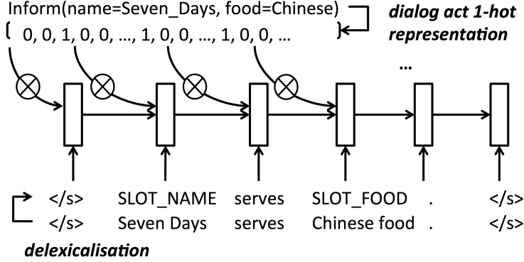
Figure 1: An unrolled view of the RNN-based generation model. It operates on a delexicalised utterance and a 1-hot encoded feature vector specified by a dialogue act type and a set of slot-value pairs. \otimes indicates the gate used for controlling the on/off states of certain feature values. The output connection layer is omitted here for simplicity.
